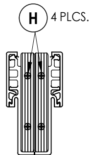
BACK-TO-BACK JAMBS END DETAIL @ Head & Sill
