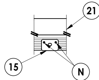
ASTRAGAL BOLT STRIKE DETAIL
